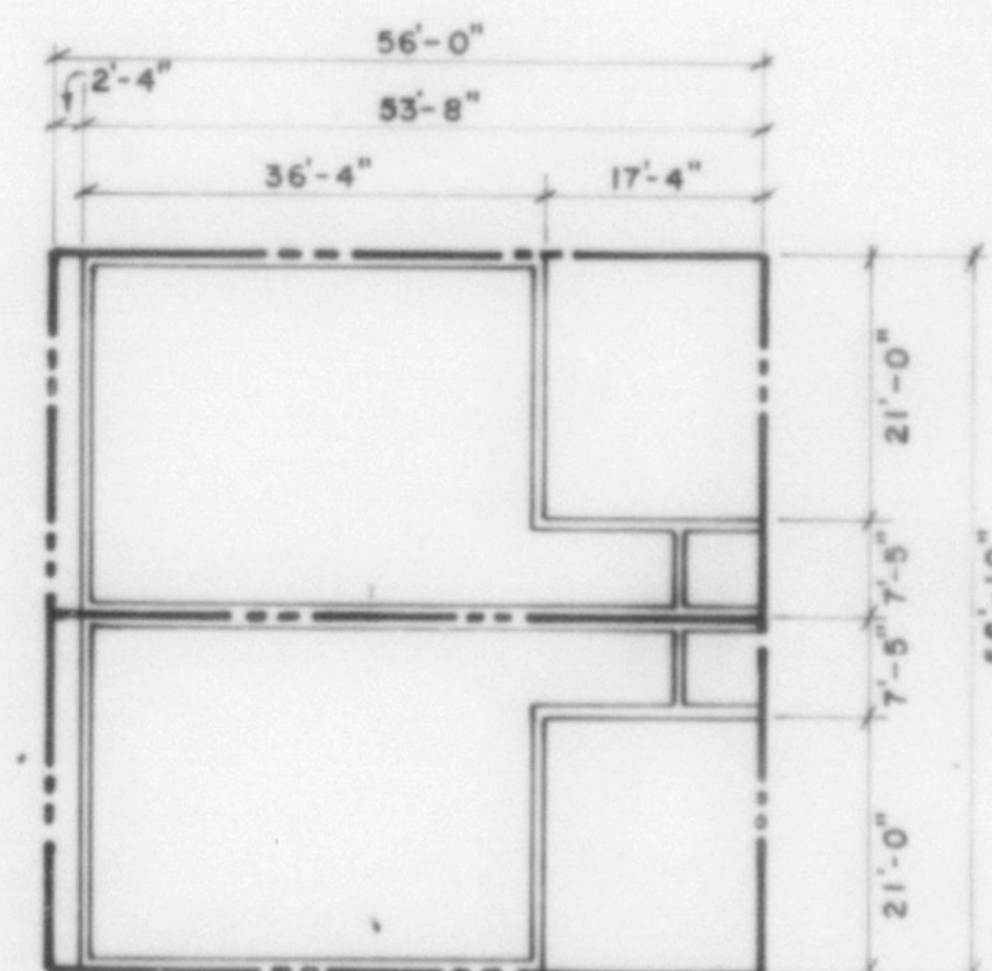
SCALE 1" = 20' TYPICAL OWNERSHIP PLAT
